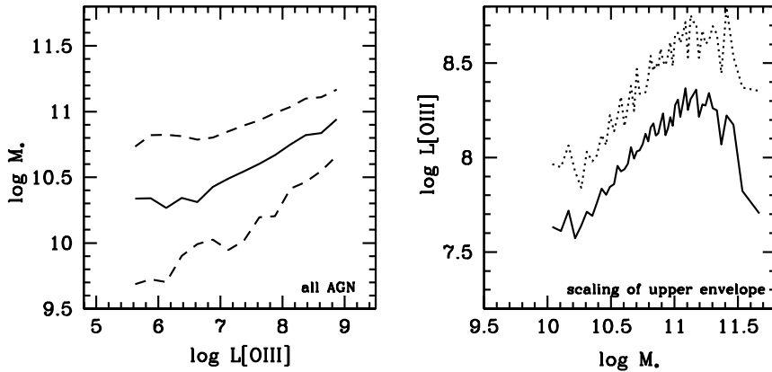
Figure 7: Left: The distribution of stellar mass as a function of [OIII] luminosity for the AGN in our sample. The solid line shows the median value of L[\text{OIII}] , while the dashed lines show the 16-84 percentiles of the 1/V_{max} weighted distribution. Right: The solid line shows the upper 97.5 percentile of the [OIII] distribution of all galaxies as a function of stellar mass. The dotted line is the upper 99 percentile.
